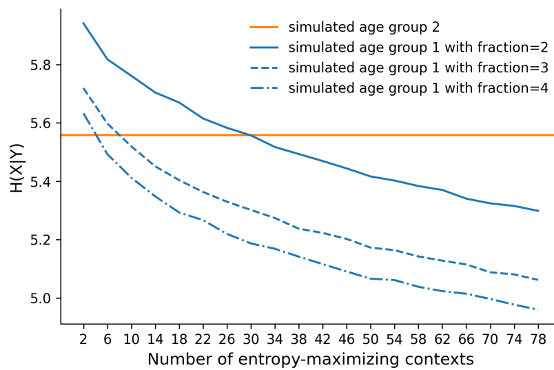
FIGURE 1.3 The relationship between H(X|Y) and the number of "entropy-maximizing" columns for artificially generated co-occurrence matrices. H(X|Y) is the conditional entropy of pseudo-nouns ( X ) given the contexts ( Y ) in which they occur. The shapes and sums of simulated co-occurrence matrices were modeled after AO-CHILDES data (650 rows and 2000 columns for age group 1; 680 rows and 2600 columns for age group 2), which allowed us to control for effects of matrix shape on entropy estimates. Simulated data was sampled either from a pseudo-Zipfian distribution (for non entropy maximizing contexts) or a random uniform distribution (for entropy-maximizing contexts). For each simulation of age group 1, we varied the fraction of co-occurrences that involve an entropy-maximizing context. Each fraction corresponds to a different line style in the figure.
