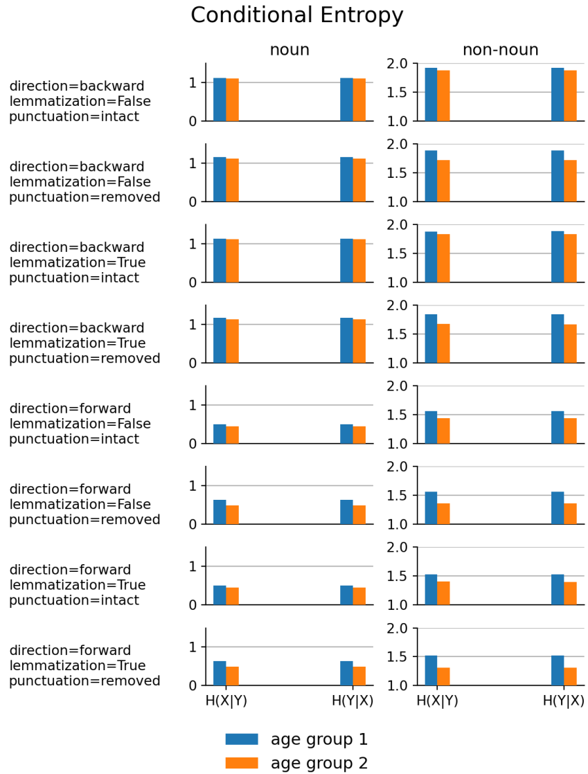
FIGURE 1.4 Comparison of conditional entropies between age group 1 and 2. Left panels are for nouns, and right panels for non-nouns. The three factors punctuation, lemmatization, and context direction are varied across rows. The y-axis units are bits.
