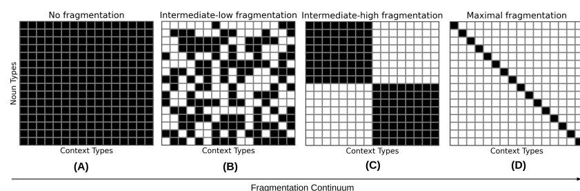
FIGURE 1.1 A visual demonstration of the fragmentation continuum, with hypothetical co-occurrence matrices (nouns in rows, contexts in columns) that exhibit either no fragmentation (A), intermediate-low fragmentation (B), intermediate-high fragmentation (C), or maximal fragmentation (D).
